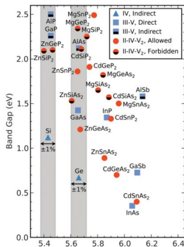
Fig. 1 Theoretically determined band gaps versus lattice constants for some of the more earth abundant II–IV–V 2 chalcopyrites. Also shown are III–V materials along with Si and Ge from group IV. The gray vertical bars overlaying Si and Ge highlight materials with similar lattice constant, within 1%
