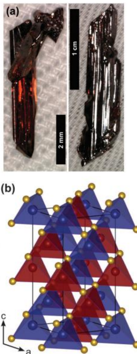
Fig. 2 (a) Photograph of ZnSiP 2 single crystals grown in Zn flux. (b) Crystal structure of II–IV–V 2 chalcopyrites (I42% d) emphasizing two interlaced networks of corner sharing tetrahedra. In one network, the tetrahedra (red) have a group IV atom at the center and group V atoms on the corners. The second network differs from the first, in that the tetrahedra (blue) are slightly distorted and they have a group II atom at the center
